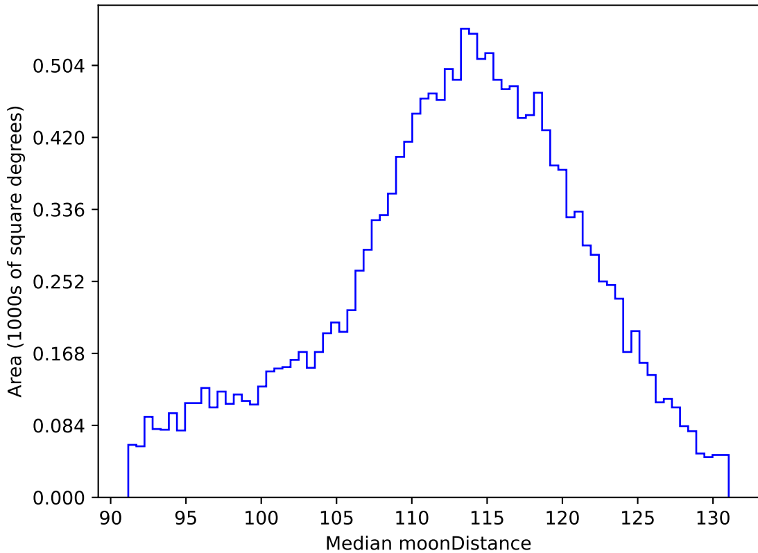
too_elab_r64_d2_ugrizy_v3.4_10yrs WFD r band: Median moonDistance
