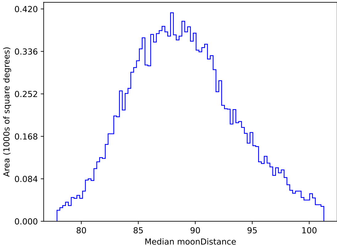
too_elab_r64_d2_ugrizy_v3.4_10yrs WFD all bands: Median moonDistance
