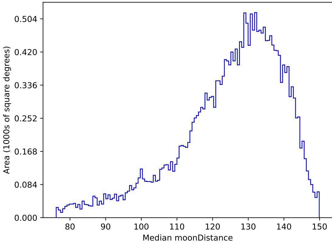
too_elab_r64_d2_ugrizy_v3.4_10yrs All sky u band: Median moonDistance
