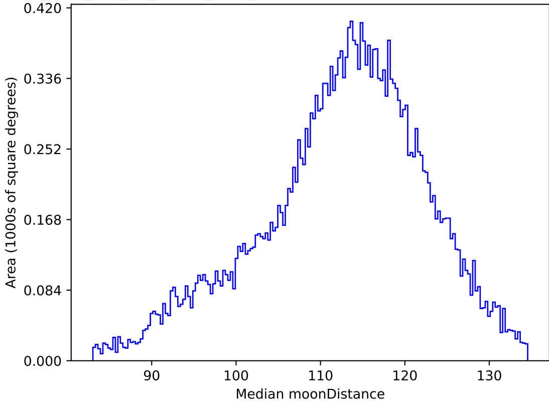
too_elab_r64_d2_ugrizy_v3.4_10yrs All sky r band: Median moonDistance
