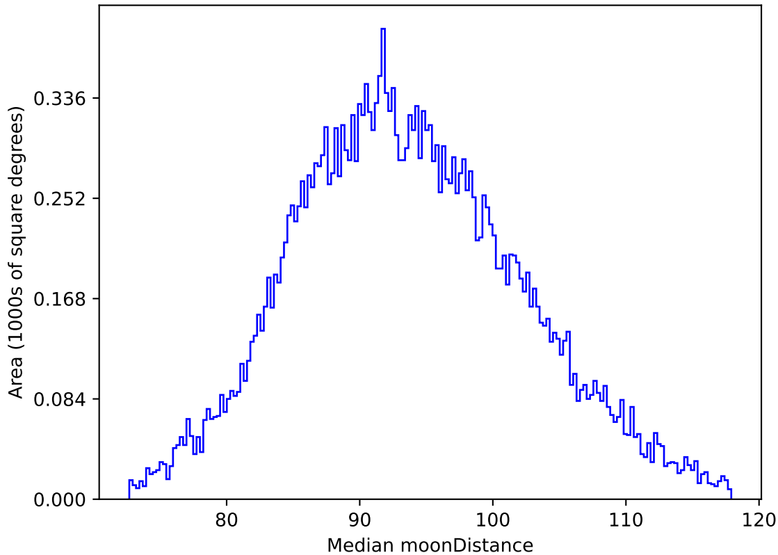
too_elab_r64_d2_ugrizy_v3.4_10yrs All sky i band: Median moonDistance
