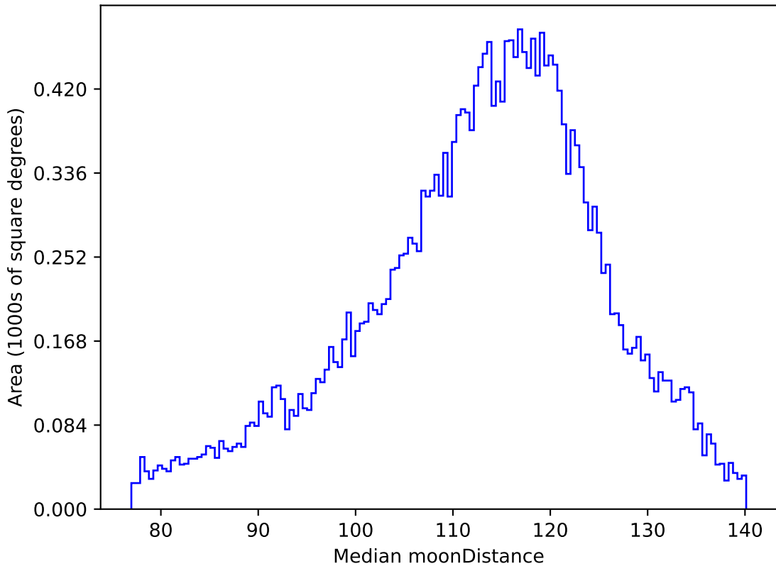
too_elab_r64_d2_ugrizy_v3.4_10yrs All sky g band: Median moonDistance
