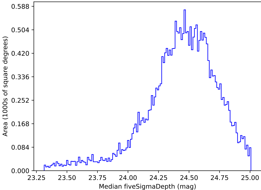
too_elab_r64_d2_ugrizy_v3.4_10yrs Yr 1 g band: Median fiveSigmaDepth
