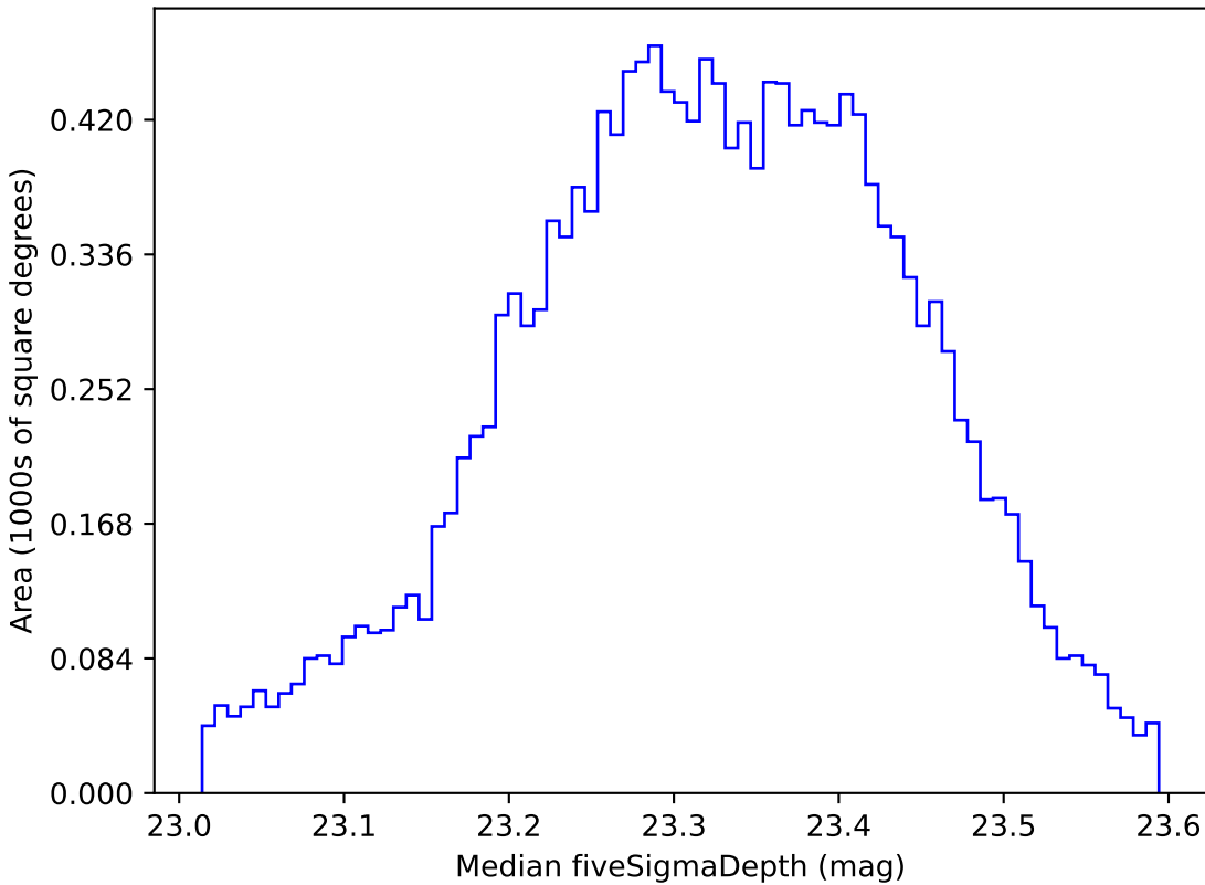
too_elab_r64_d2_ugrizy_v3.4_10yrs WFD all bands: Median fiveSigmaDepth
