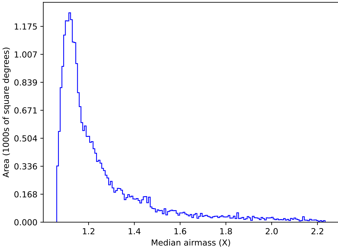
too_elab_r64_d2_ugrizy_v3.4_10yrs Yr 1 z band: Median airmass
