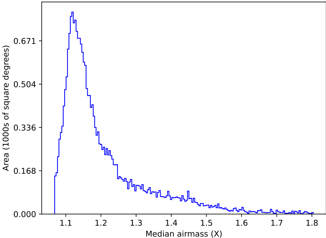
too_elab_r64_d2_ugrizy_v3.4_10yrs Yr 1 y band: Median airmass
