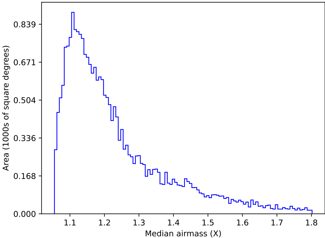
too_elab_r64_d2_ugrizy_v3.4_10yrs Yr 1 u band: Median airmass
