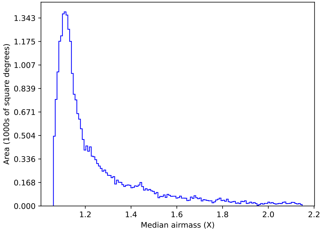
too_elab_r64_d2_ugrizy_v3.4_10yrs Yr 1 r band: Median airmass
