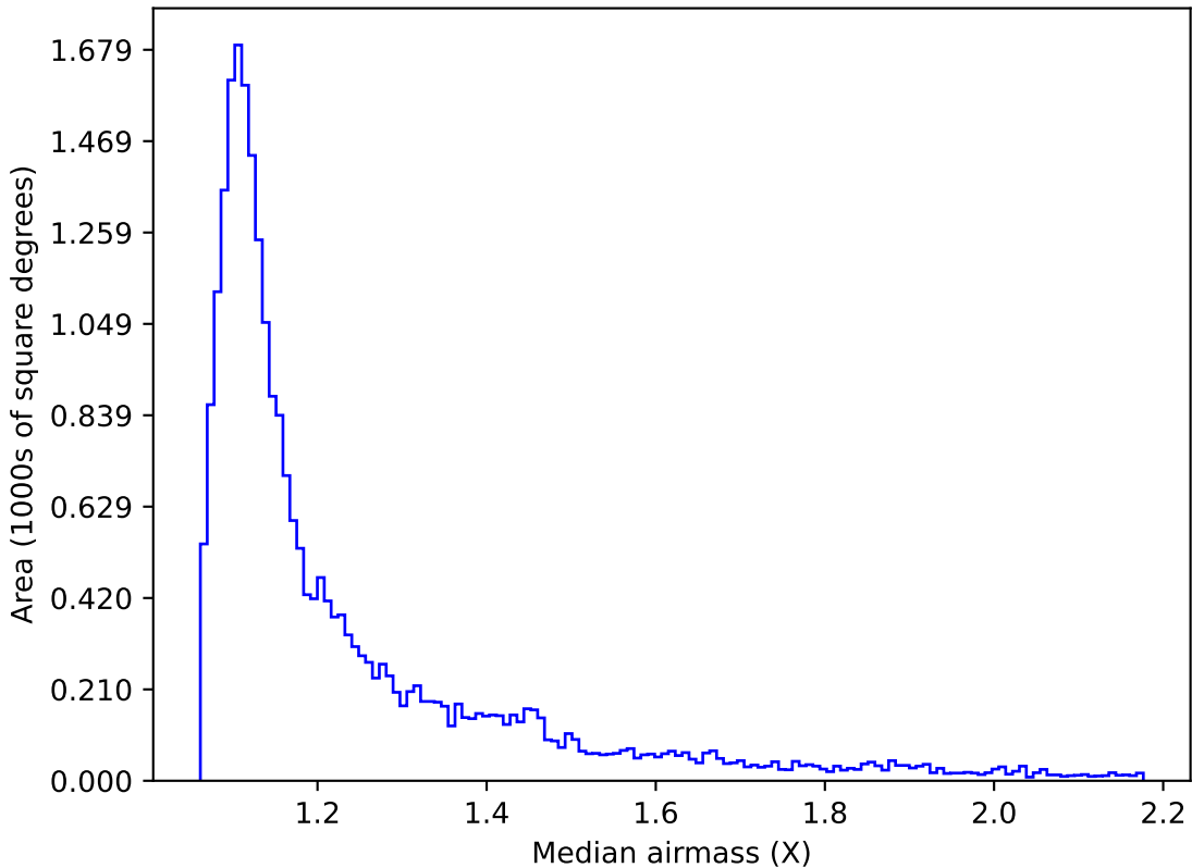
too_elab_r64_d2_ugrizy_v3.4_10yrs Yr 1 i band: Median airmass
