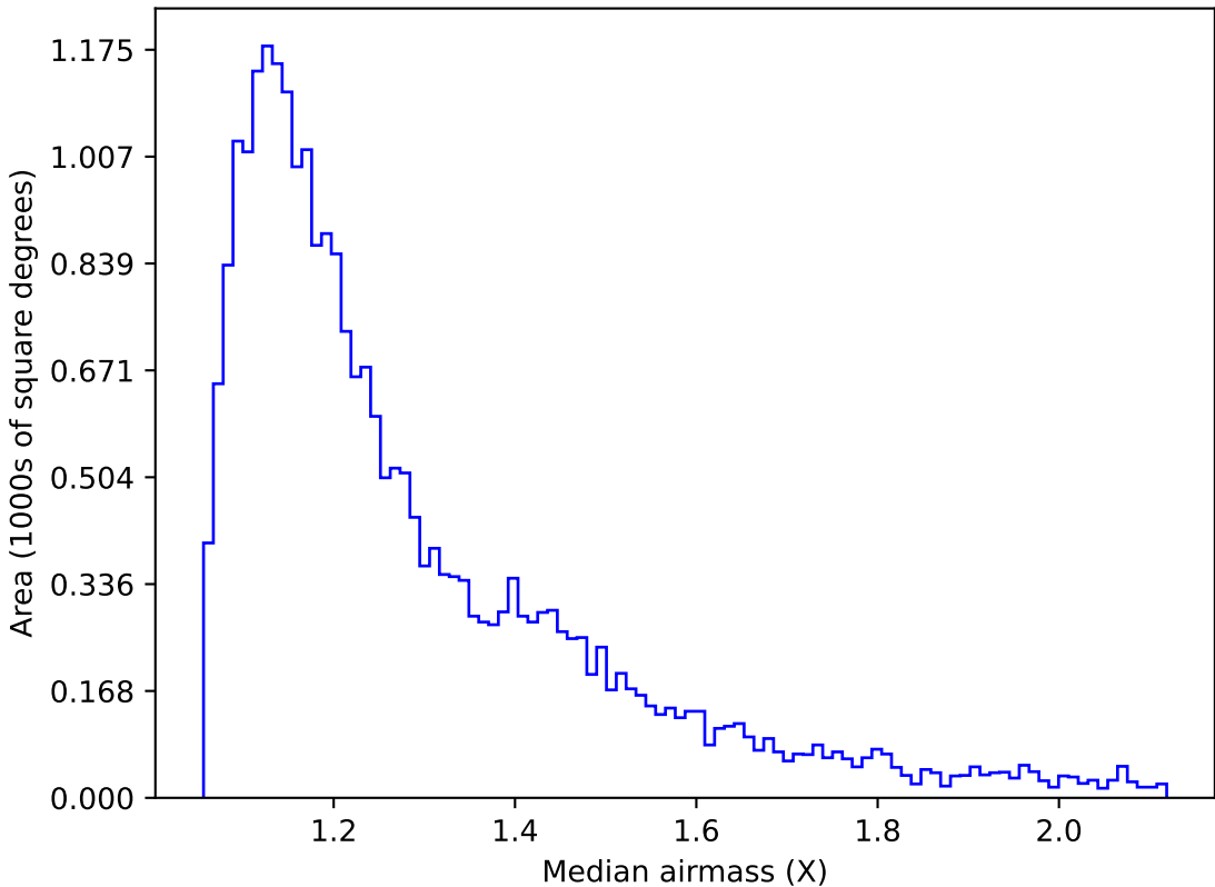
too_elab_r64_d2_ugrizy_v3.4_10yrs Yr 1 g band: Median airmass
