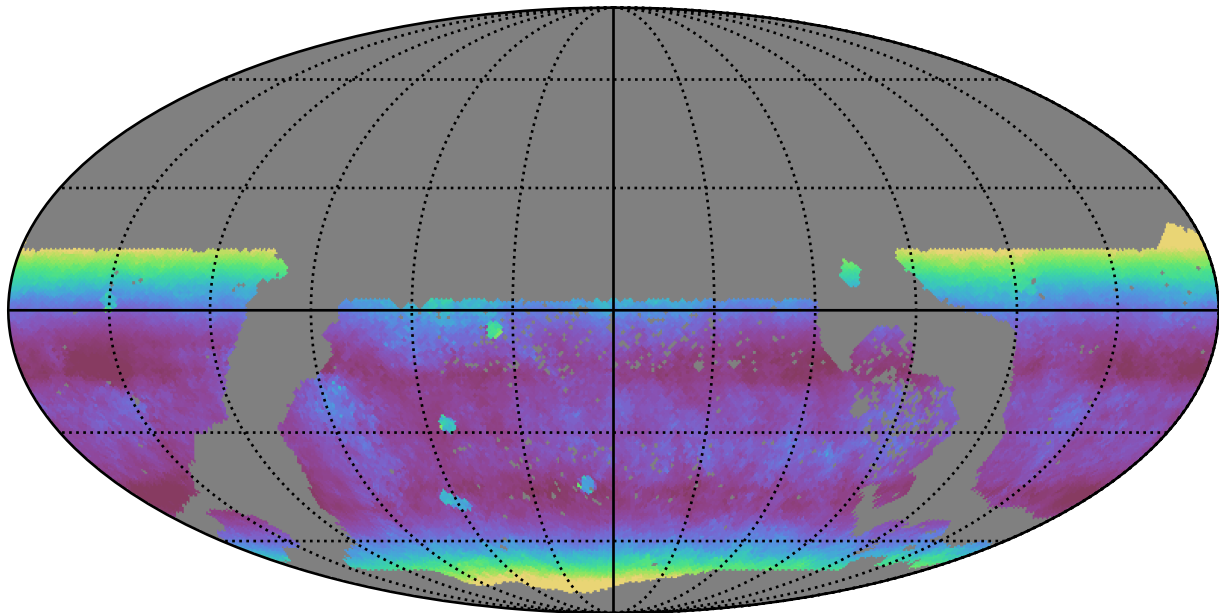
too_elab_r64_d2_ugrizy_v3.4_10yrs WFD z band: Median airmass
