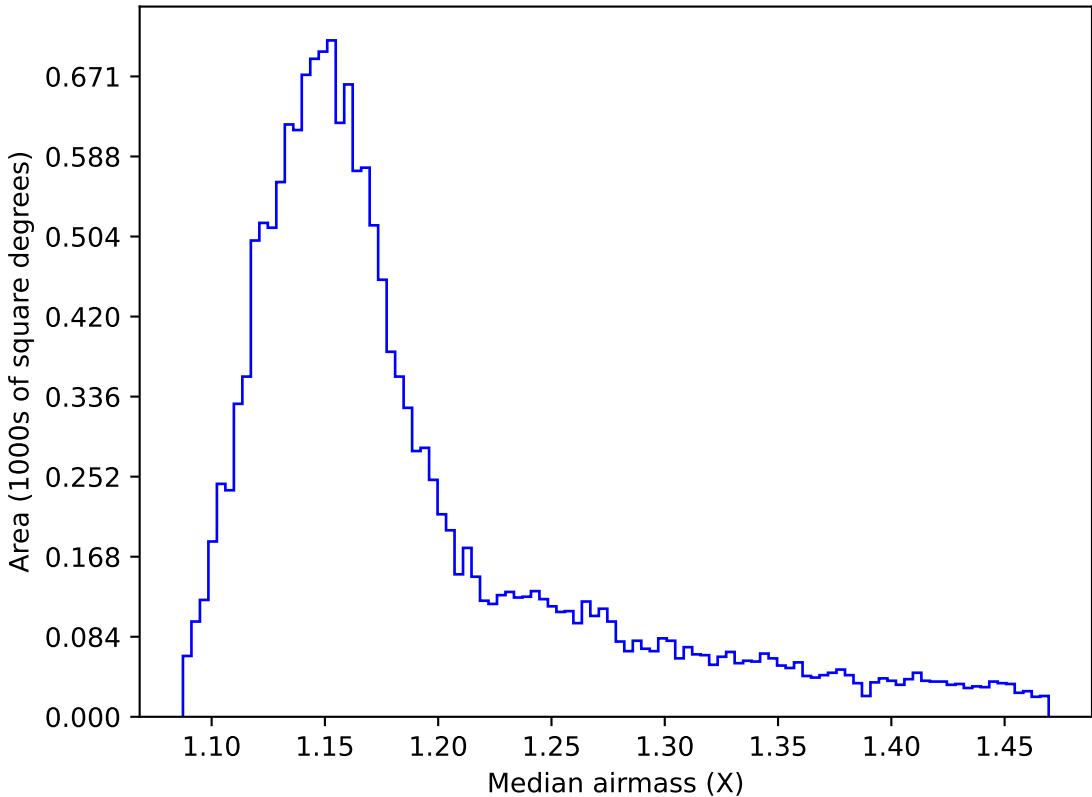
too_elab_r64_d2_ugrizy_v3.4_10yrs WFD z band: Median airmass
