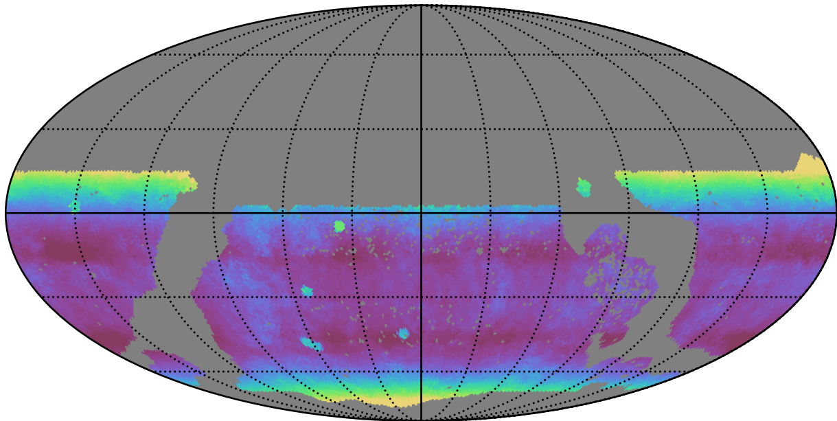
too_elab_r64_d2_ugrizy_v3.4_10yrs WFD y band: Median airmass
