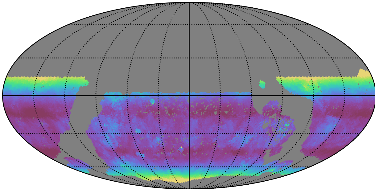
too_elab_r64_d2_ugrizy_v3.4_10yrs WFD u band: Median airmass
