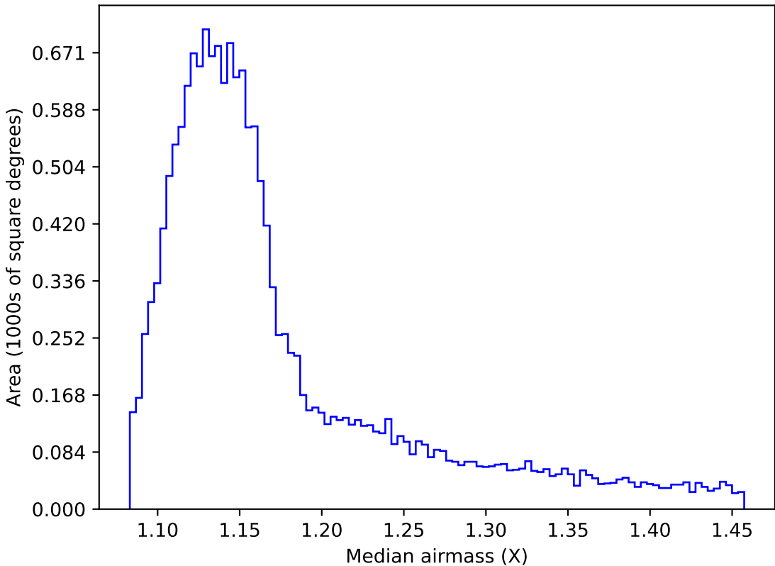
too_elab_r64_d2_ugrizy_v3.4_10yrs WFD i band: Median airmass
