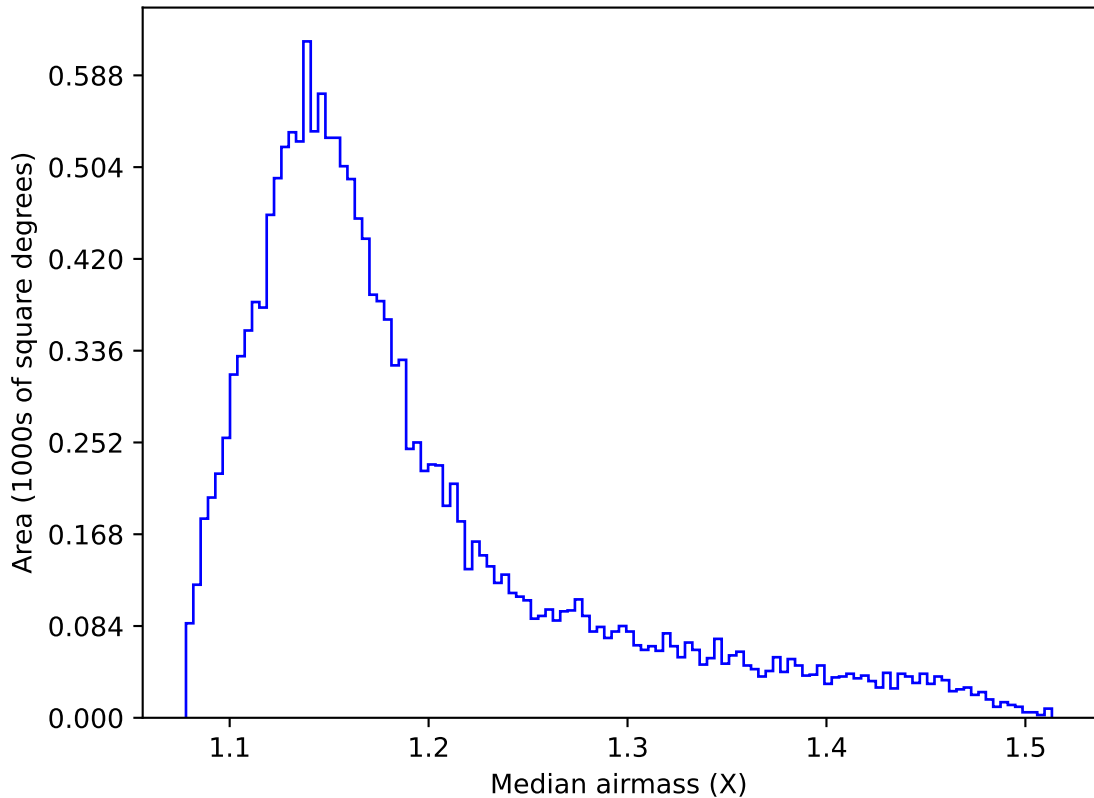
too_elab_r64_d2_ugrizy_v3.4_10yrs WFD g band: Median airmass
