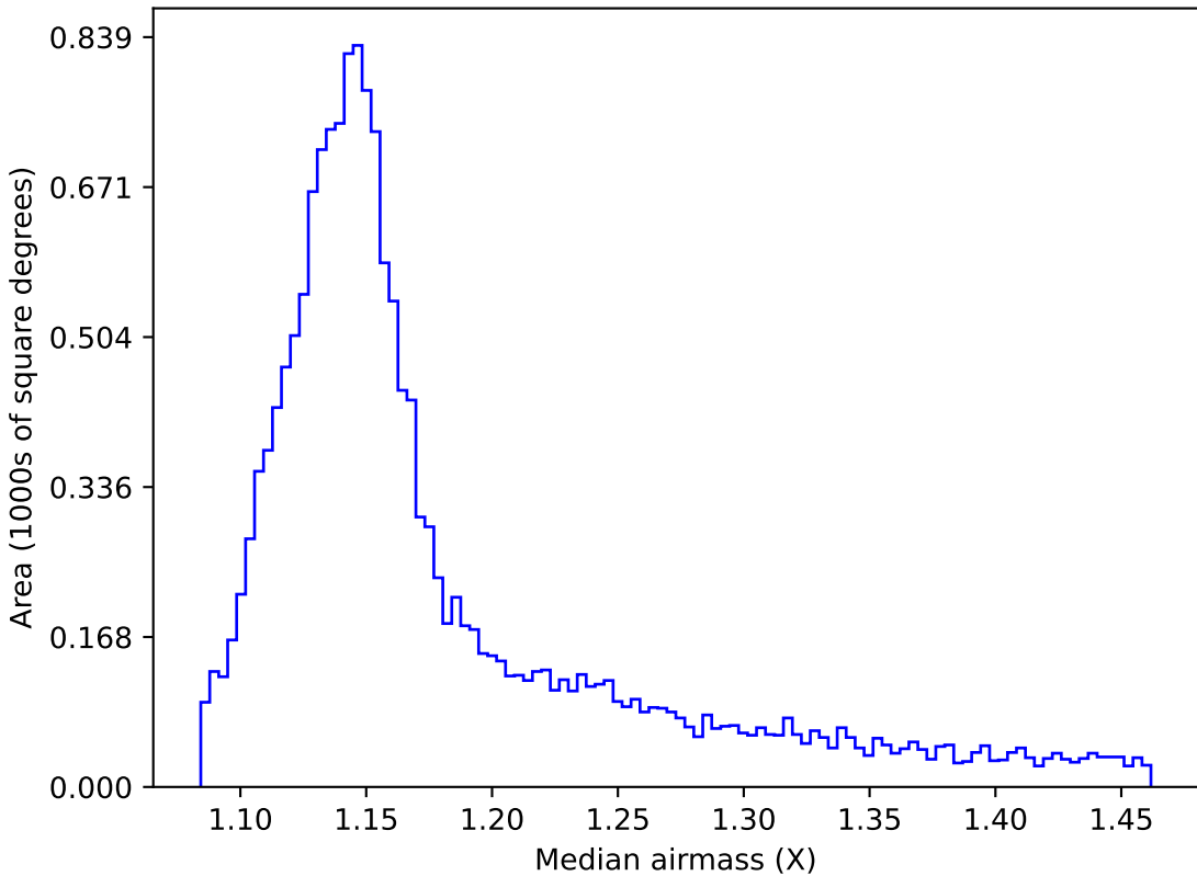
too_elab_r64_d2_ugrizy_v3.4_10yrs WFD all bands: Median airmass
