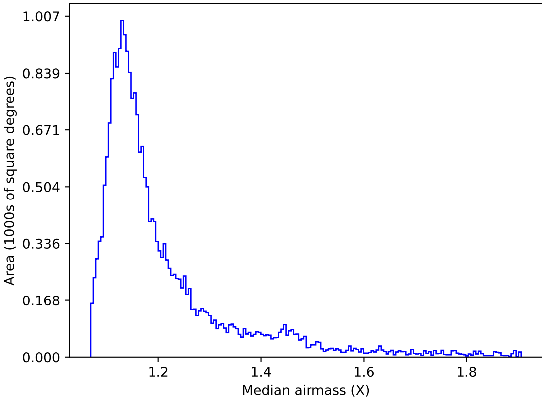
too_elab_r64_d2_ugrizy_v3.4_10yrs All sky u band: Median airmass
