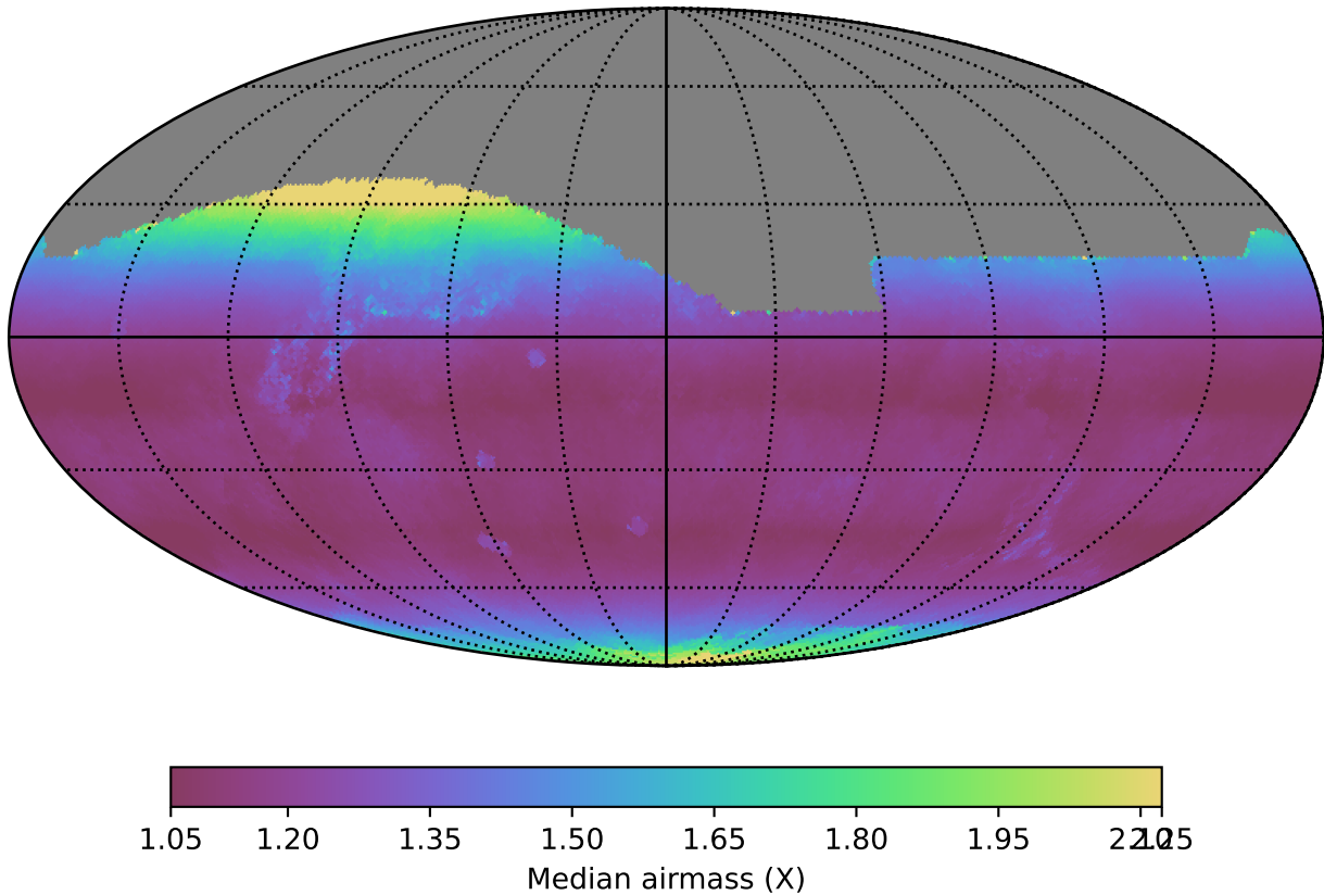
too_elab_r64_d2_ugrizy_v3.4_10yrs All sky r band: Median airmass
