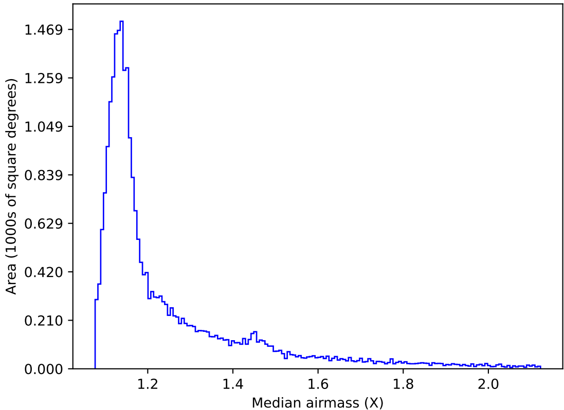
too_elab_r64_d2_ugrizy_v3.4_10yrs All sky r band: Median airmass
