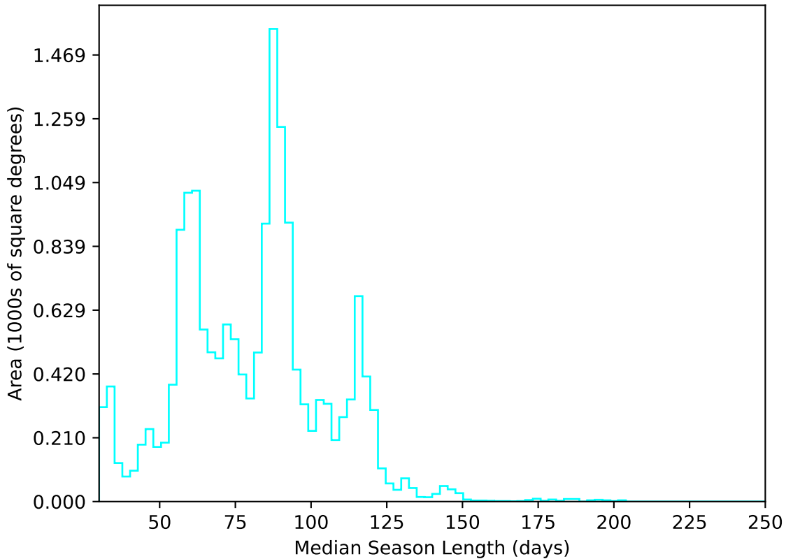
too_elab_r64_d2_ugrizy_v3.4_10yrs WFD u band: Median Season Length
