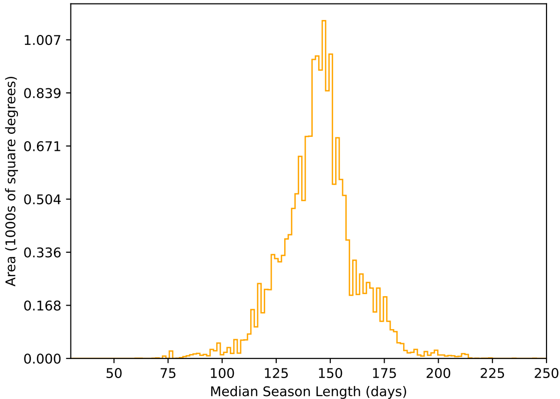
too_elab_r64_d2_ugrizy_v3.4_10yrs WFD r band: Median Season Length
