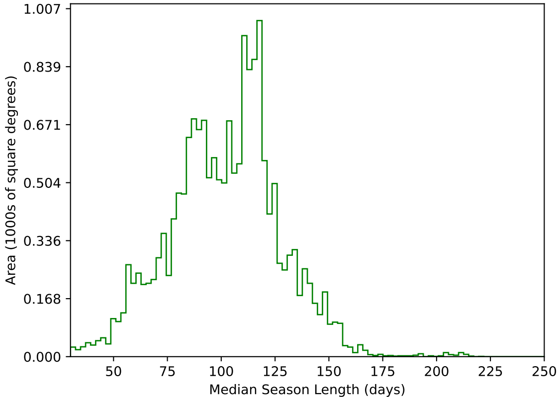
too_elab_r64_d2_ugrizy_v3.4_10yrs WFD g band: Median Season Length
