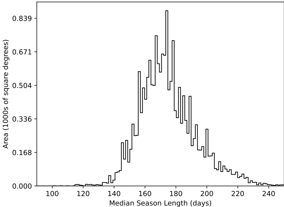
too_elab_r64_d2_ugrizy_v3.4_10yrs WFD all bands: Median Season Length
