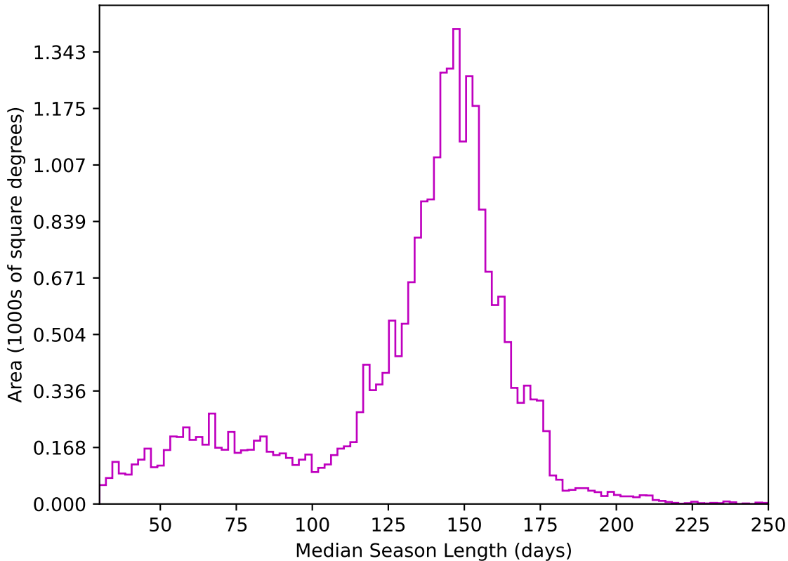
too_elab_r64_d2_ugrizy_v3.4_10yrs All sky z band: Median Season Length
