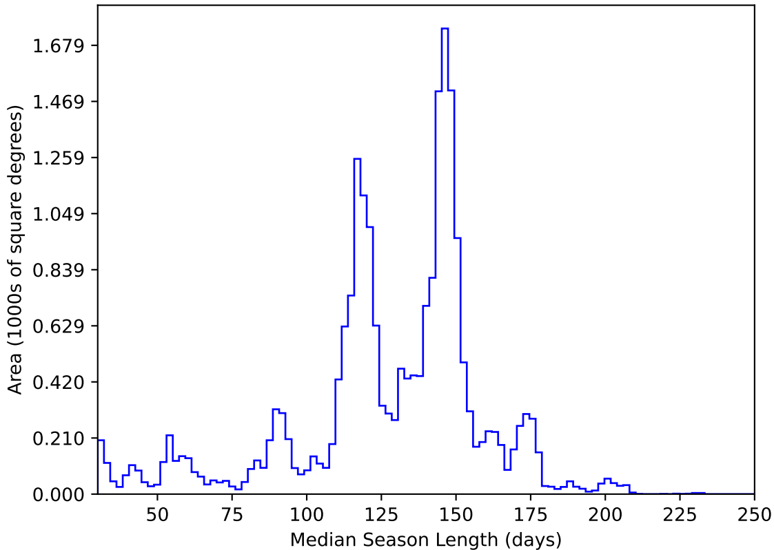
too_elab_r64_d2_ugrizy_v3.4_10yrs All sky y band: Median Season Length
