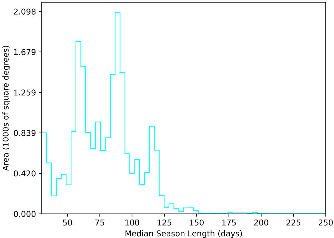
too_elab_r64_d2_ugrizy_v3.4_10yrs All sky u band: Median Season Length
