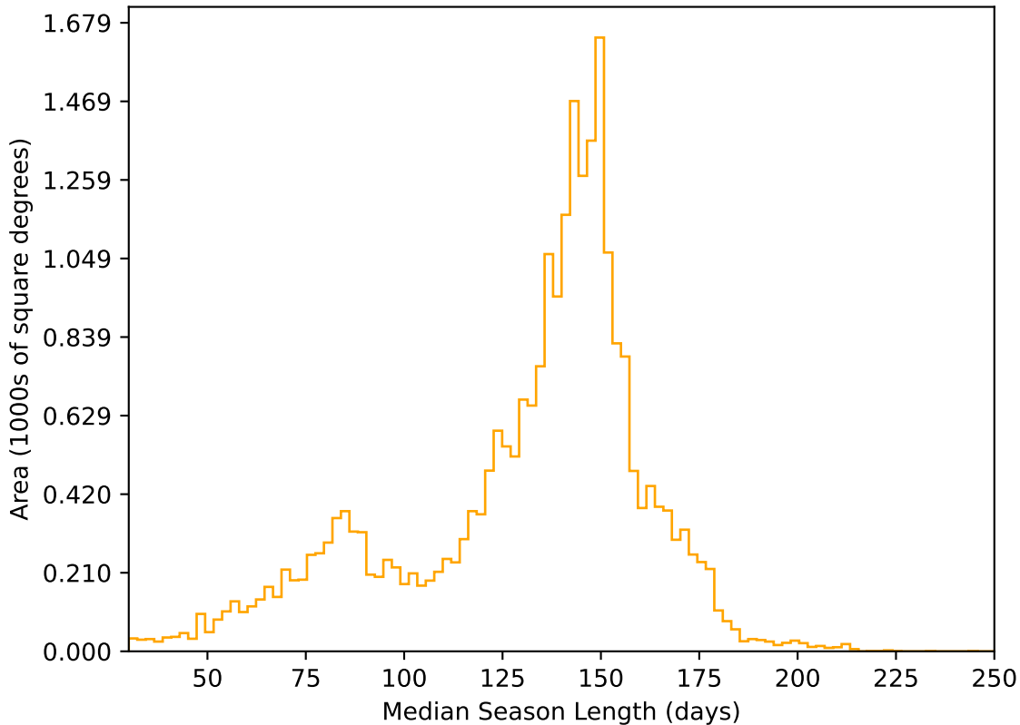
too_elab_r64_d2_ugrizy_v3.4_10yrs All sky r band: Median Season Length
