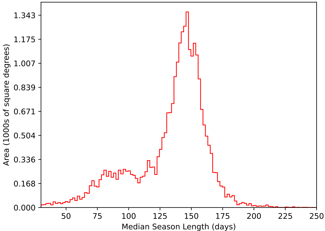
too_elab_r64_d2_ugrizy_v3.4_10yrs All sky i band: Median Season Length
