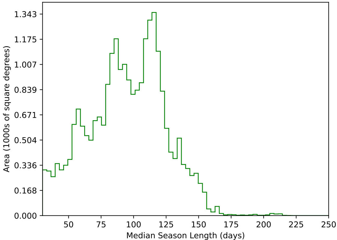
too_elab_r64_d2_ugrizy_v3.4_10yrs All sky g band: Median Season Length
