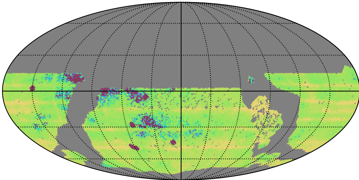
too_elab_r64_d2_ugrizy_v3.4_10yrs WFD: Median Intra-Night Gap
