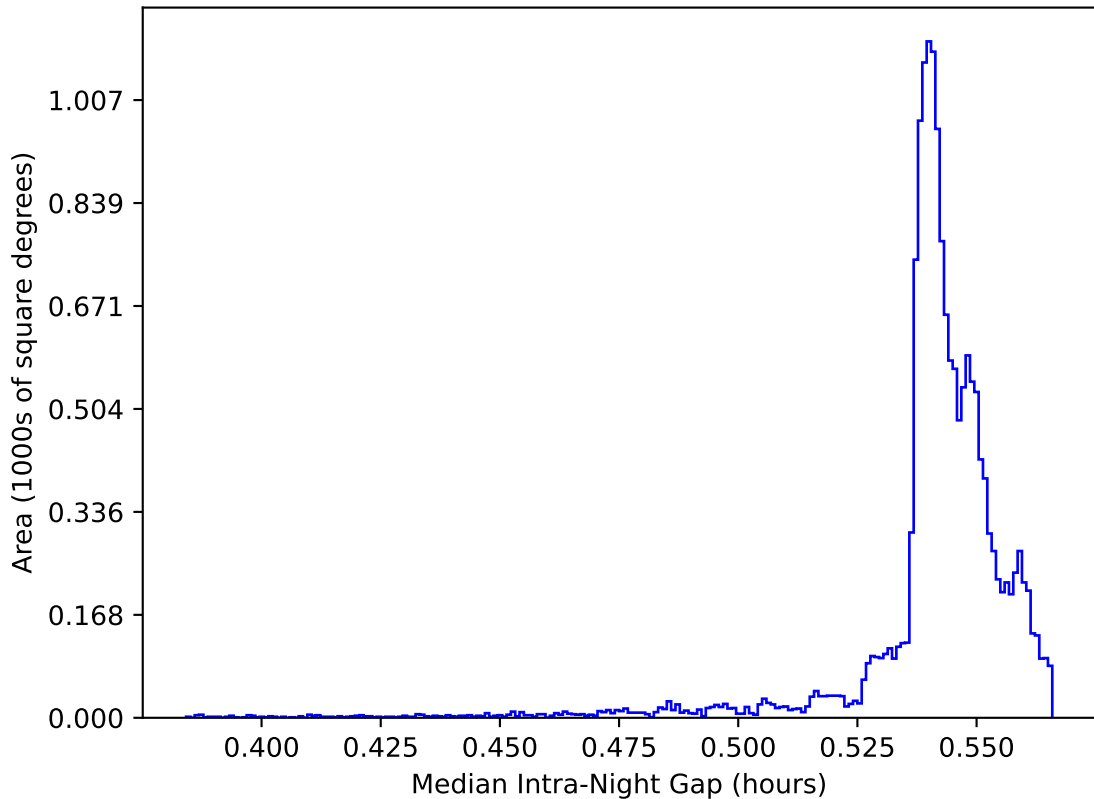
too_elab_r64_d2_ugrizy_v3.4_10yrs WFD: Median Intra-Night Gap
