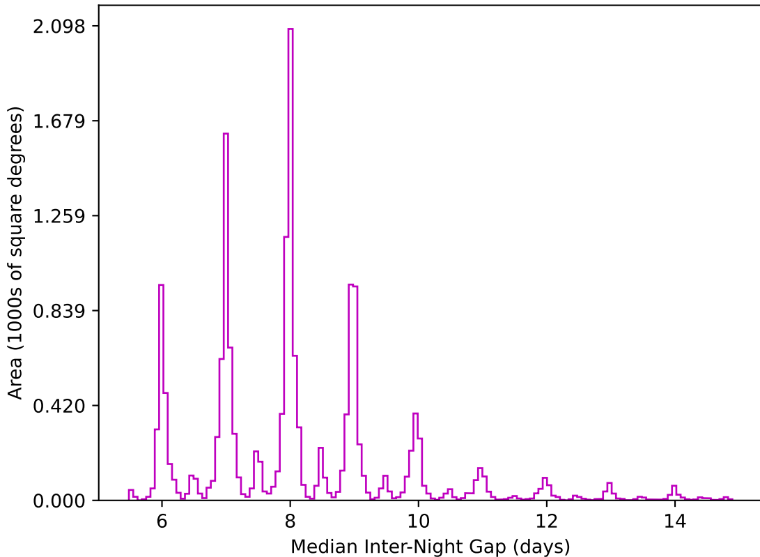
too_elab_r64_d2_ugrizy_v3.4_10yrs WFD z band: Median Inter-Night Gap
