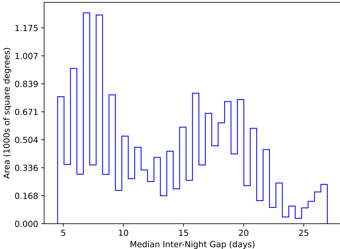
too_elab_r64_d2_ugrizy_v3.4_10yrs WFD y band: Median Inter-Night Gap
