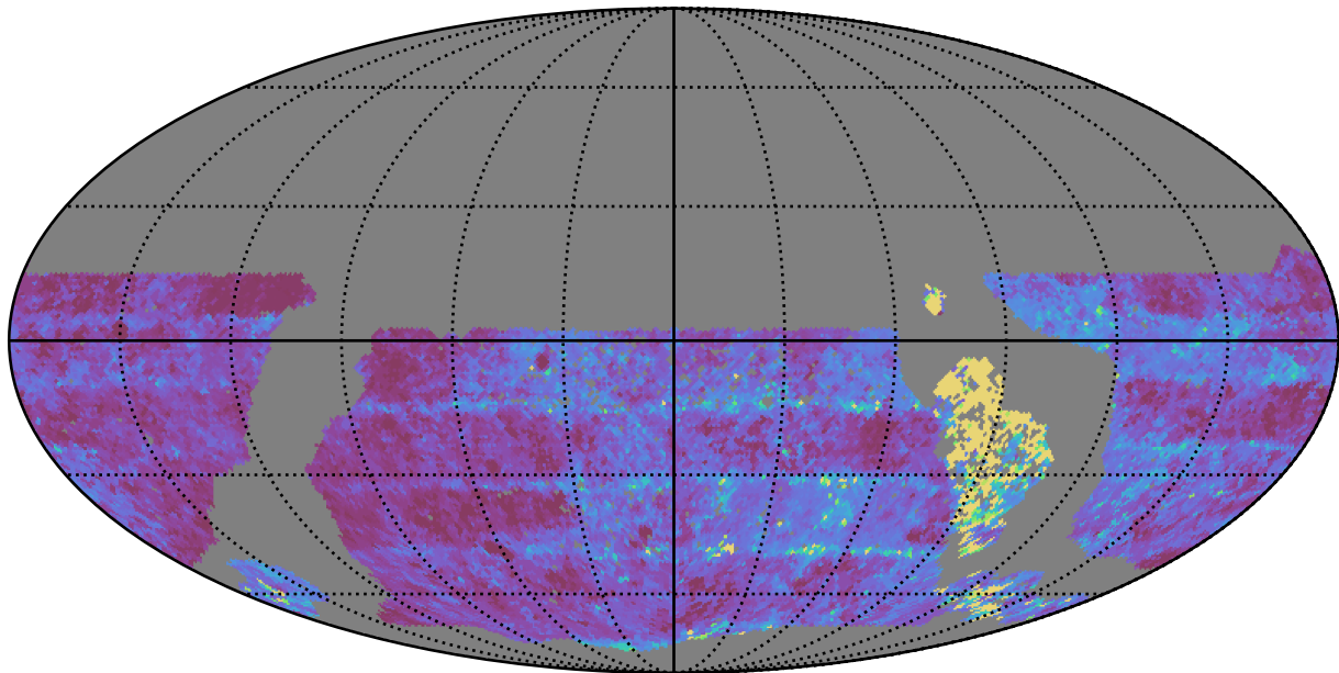
too_elab_r64_d2_ugrizy_v3.4_10yrs WFD u band: Median Inter-Night Gap
