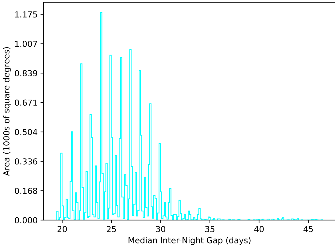
too_elab_r64_d2_ugrizy_v3.4_10yrs WFD u band: Median Inter-Night Gap
