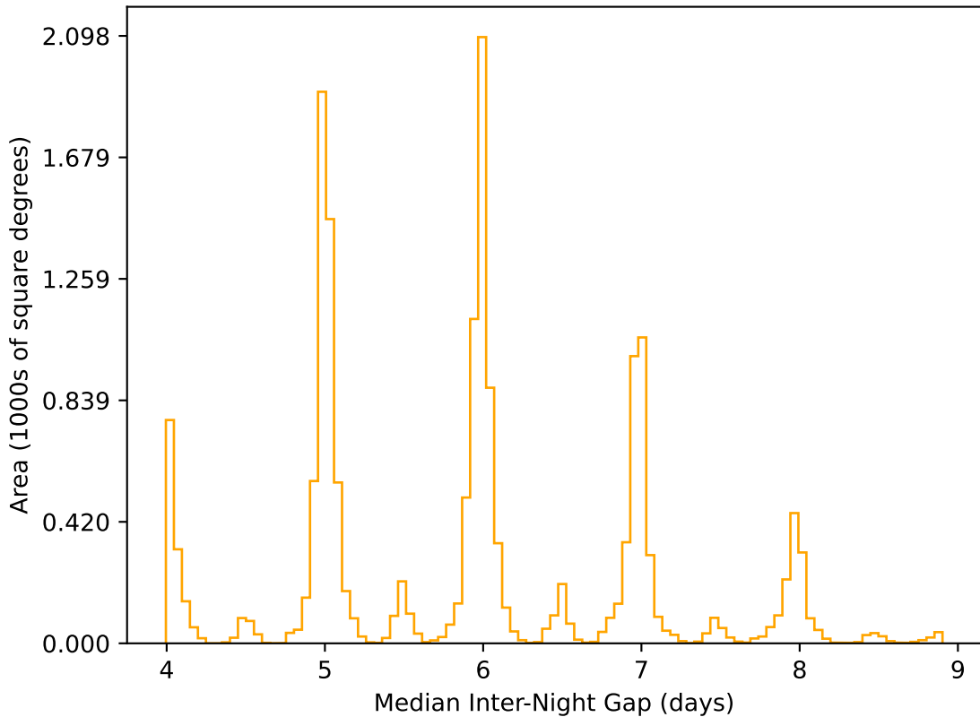
too_elab_r64_d2_ugrizy_v3.4_10yrs WFD r band: Median Inter-Night Gap
