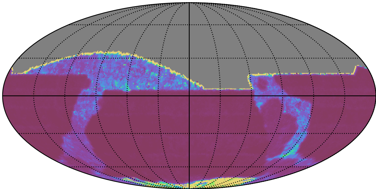
too_elab_r64_d2_ugrizy_v3.4_10yrs All sky z band: Median Inter-Night Gap
