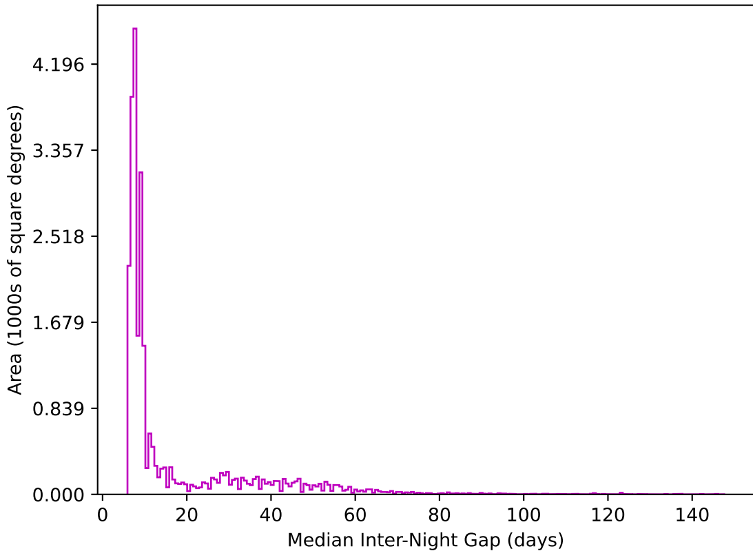
too_elab_r64_d2_ugrizy_v3.4_10yrs All sky z band: Median Inter-Night Gap
