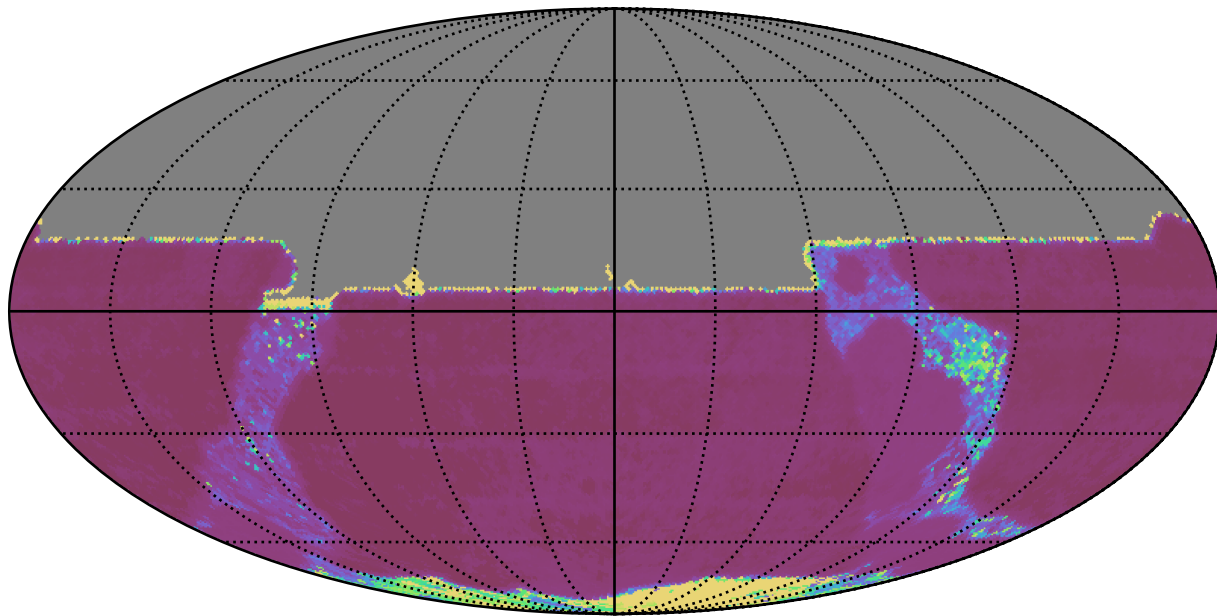
too_elab_r64_d2_ugrizy_v3.4_10yrs All sky y band: Median Inter-Night Gap
