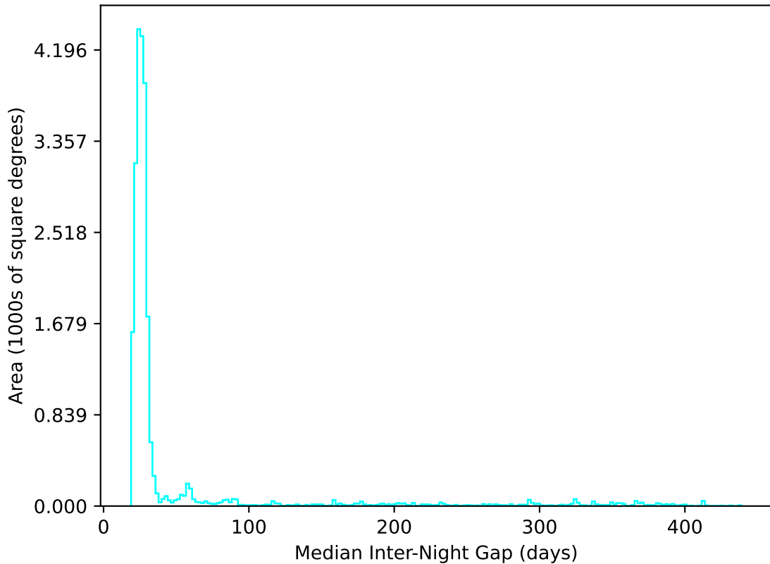
too_elab_r64_d2_ugrizy_v3.4_10yrs All sky u band: Median Inter-Night Gap
