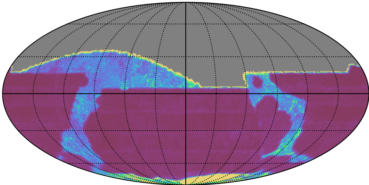
too_elab_r64_d2_ugrizy_v3.4_10yrs All sky r band: Median Inter-Night Gap
