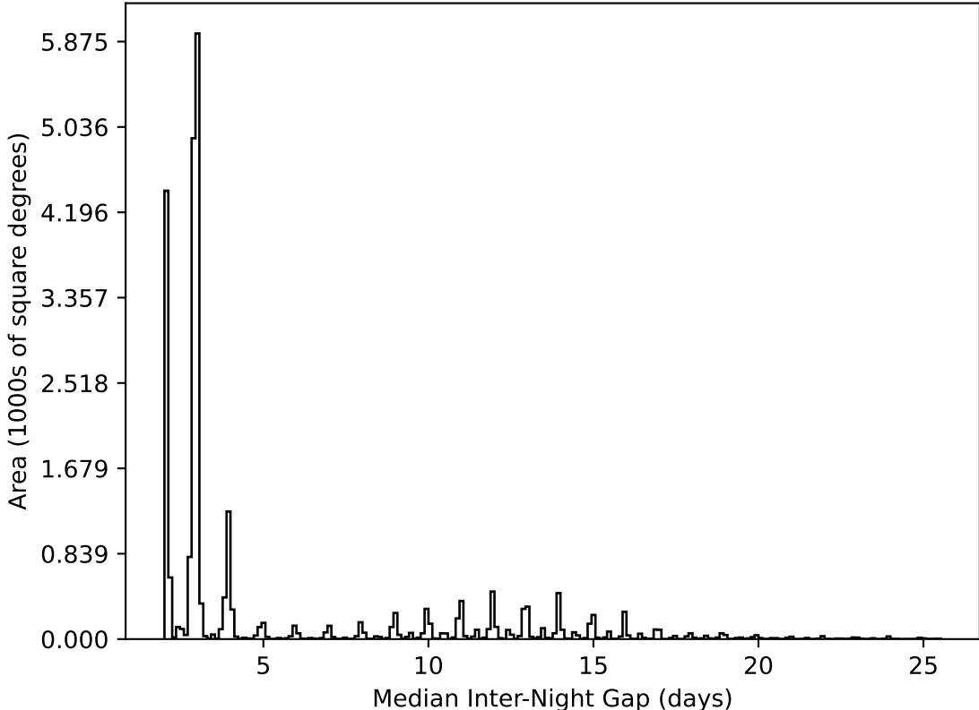
too_elab_r64_d2_ugrizy_v3.4_10yrs All sky all bands: Median Inter-Night Gap
