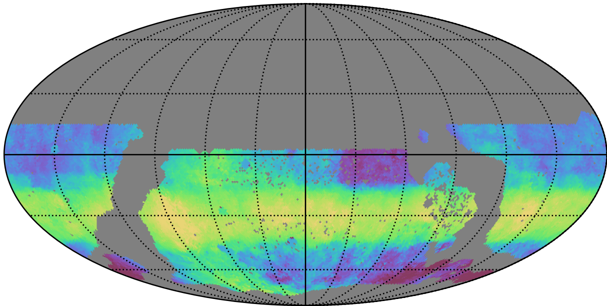
too_elab_r64_d2_ugrizy_v3.4_10yrs WFD z band: Median HA
