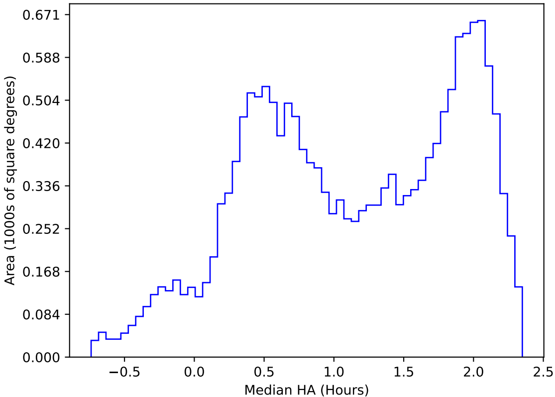
too_elab_r64_d2_ugrizy_v3.4_10yrs WFD z band: Median HA
