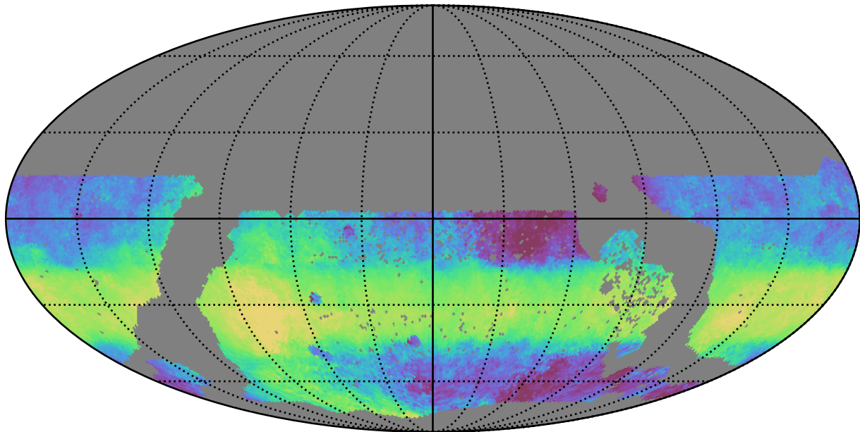
too_elab_r64_d2_ugrizy_v3.4_10yrs WFD y band: Median HA
